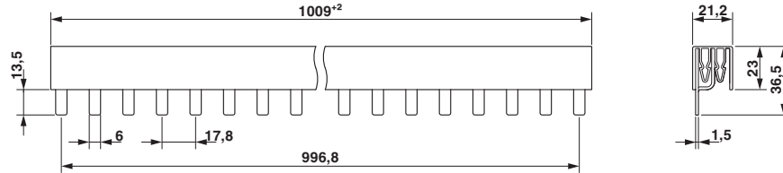
Dimensional drawing
